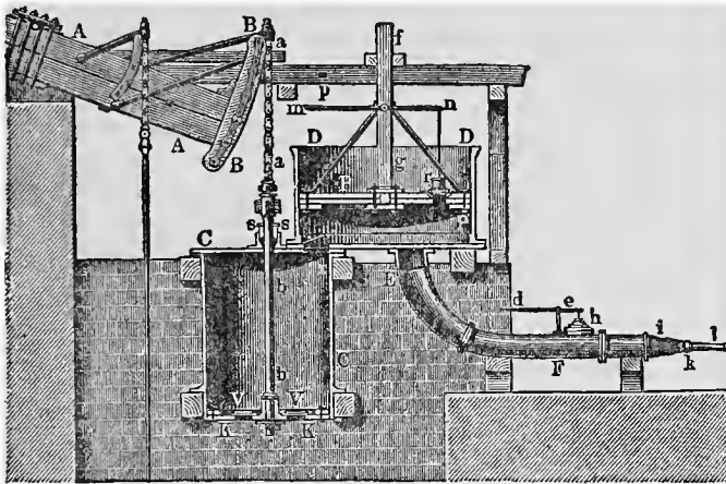
FIG. 10. DEVELOPED CYLINDRICAL BLOWING ENGINE
